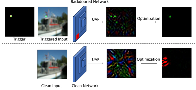
Figure 4.2: The structure of USB. First, we generate targeted UAP for the clean model and the backdoored model. Second, we optimize UAPs to reverse engineer the potential trigger. The pixel values of the two UAPs are scaled for visibility.
